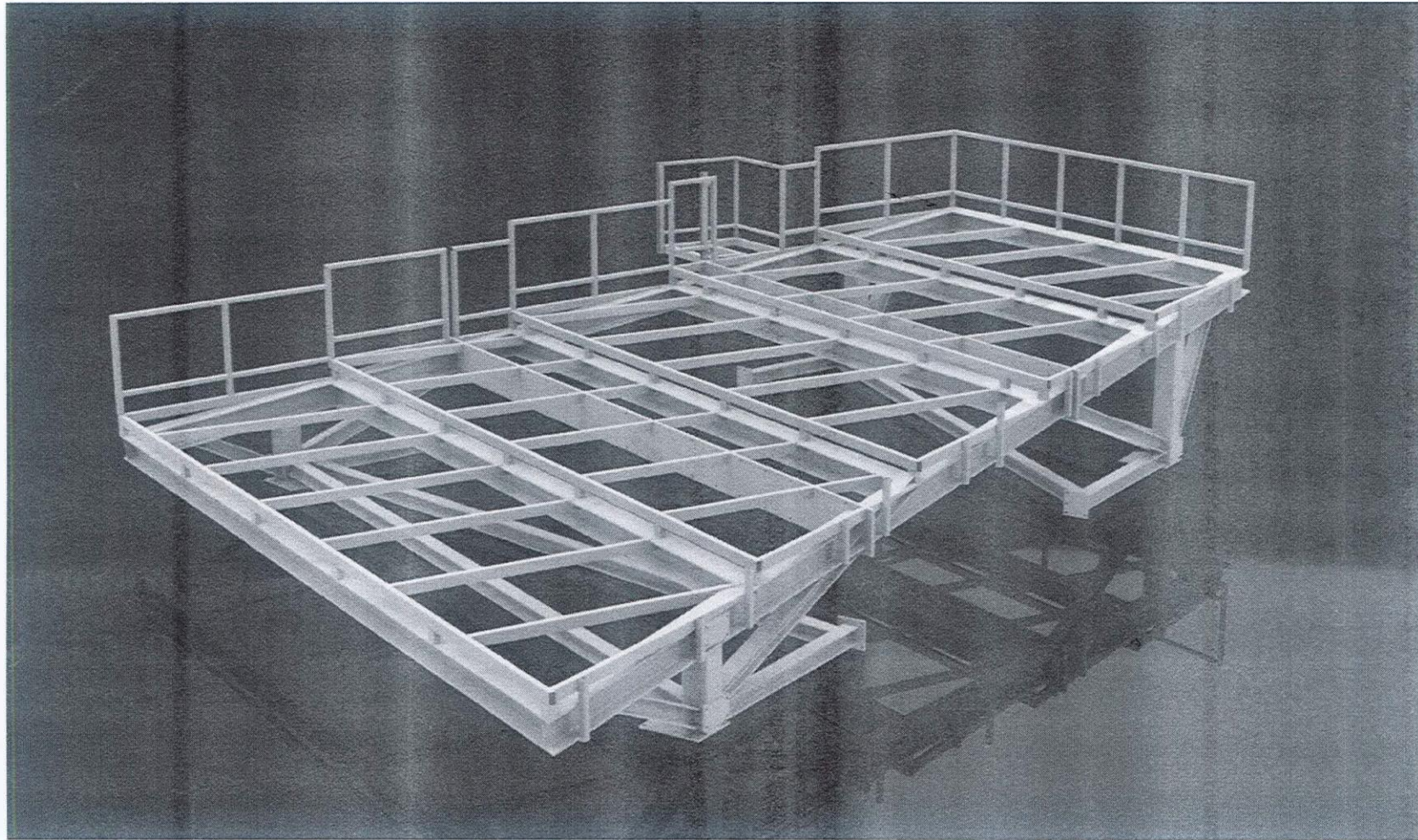
Aircraft Wing Docking • Basic Frame Design
